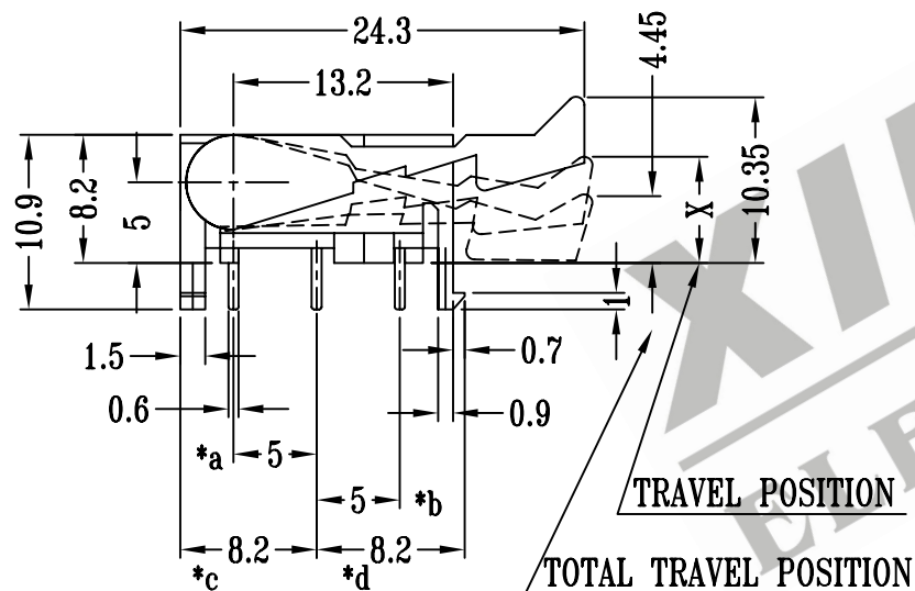
P.C.B.MOUNTING FACE OPERATING FORCE: 50±20 gf
