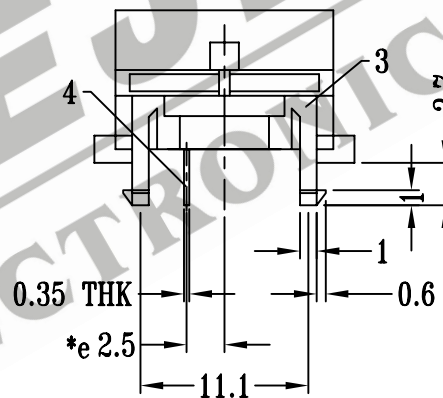
P.C.B.MOUNTING FACE OPERATING FORCE: 50±20 gf
